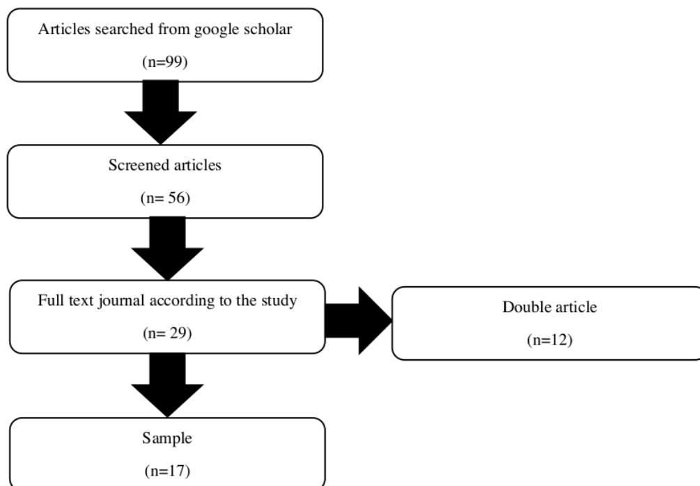
Figure 1. Scheme of Selection Method
