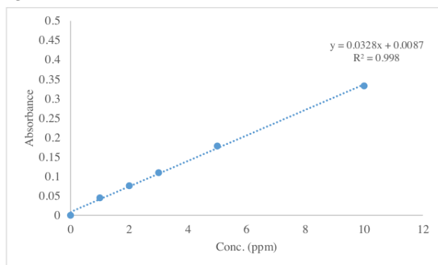
Figure 2. Linearity plot of calcium standard solution by atomic absorption spectroscopic
